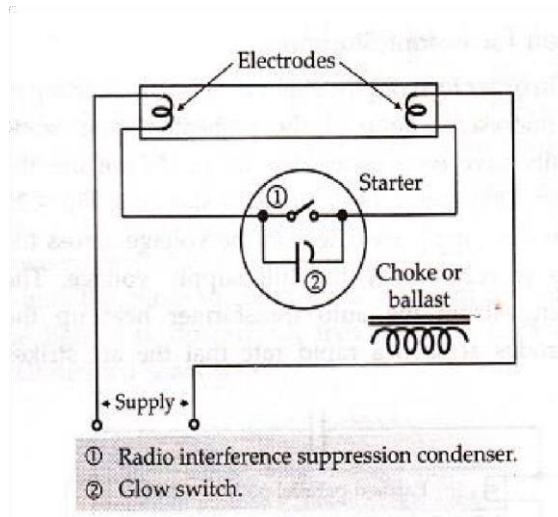
Fig.9 Fluorescent lamp
