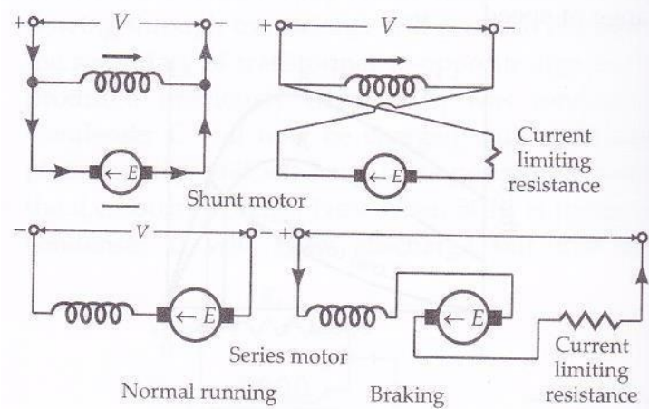
Fig.21 Plugging in DC motors
