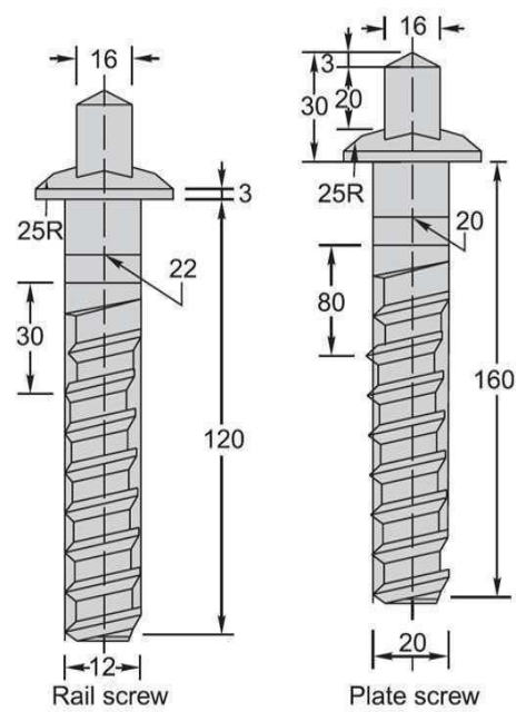
Screw spikes
