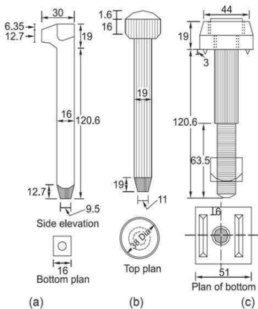
(a) Dog spike, (b) round spike, (c) fang bolt
