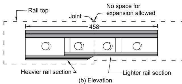
Combination fish plate (dimensions in mm)
